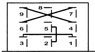
MRC, WIRE JUMPER DETAIL 1 TO 3, 2 TO 5, 4 TO 9, 6 TO 7
