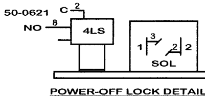
POWER-OFF LOCK DETAIL
