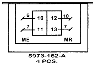
MRC, BOTTOM VIEW
