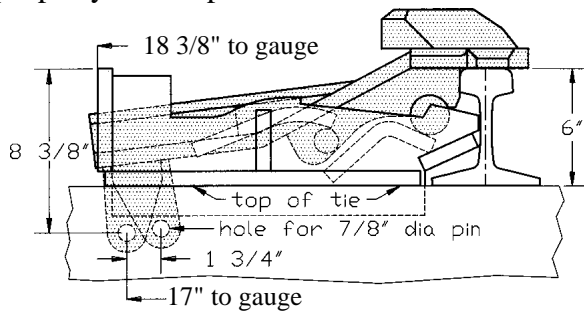
Model HB Size 6 on 6" Rail
